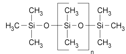
Polydimethylsiloxan PDMS
