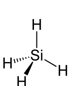
Monosilan
