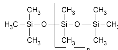
Polydimethylsiloxan PDMS
