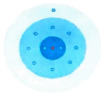
2 Natrium-Atom
