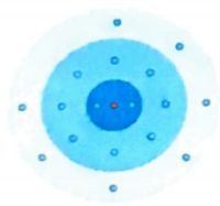
3 Chlor-Atom
