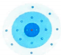
3 Chlor-Atom
