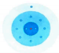
2 Natrium-Atom
