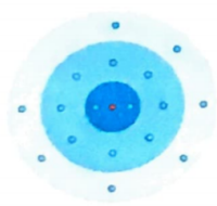
3 Chlor-Atom
