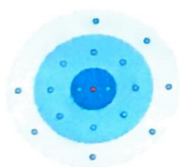
3 Chlor-Atom
