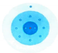
2 Natrium-Atom
