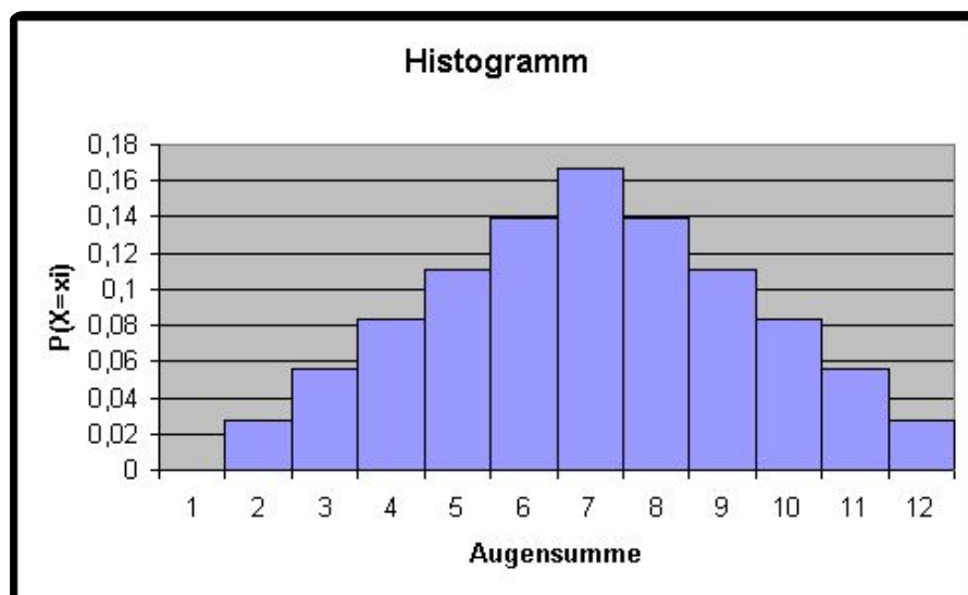
Histogramm Augensumme
