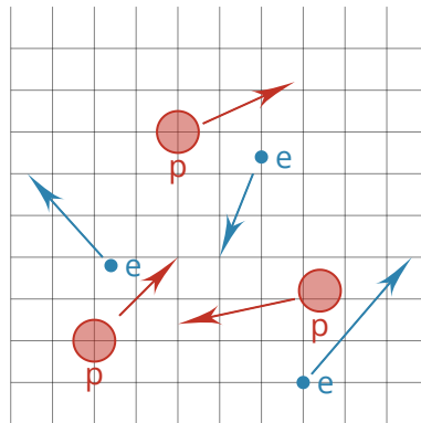
Plasma
